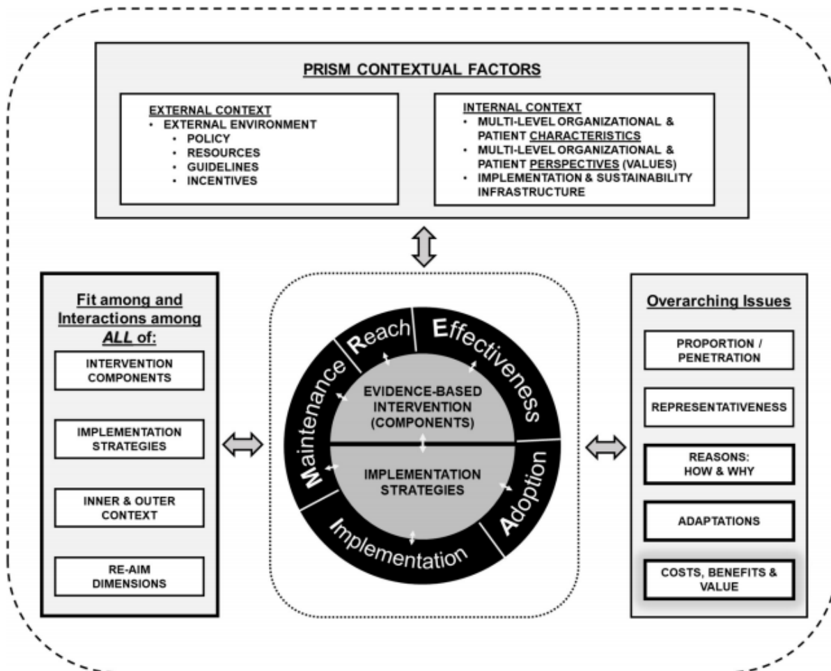
Figure 1. PRISM/RE-AIM Framework
